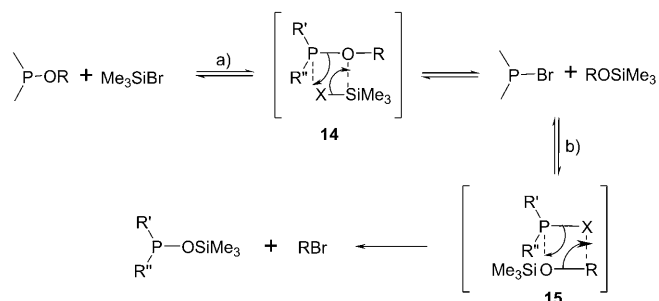
Scheme 13.
