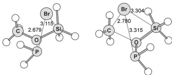
Figure 1. Transition state geometries for \text{H}_2\text{POMe}+\text{H}_3\text{SiBr} and \text{H}_3\text{PBr}+\text{H}_3\text{SiOMe} reactions, respectively.
